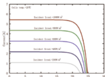
I-V Curves of SPP105QH36S at different irradiance
